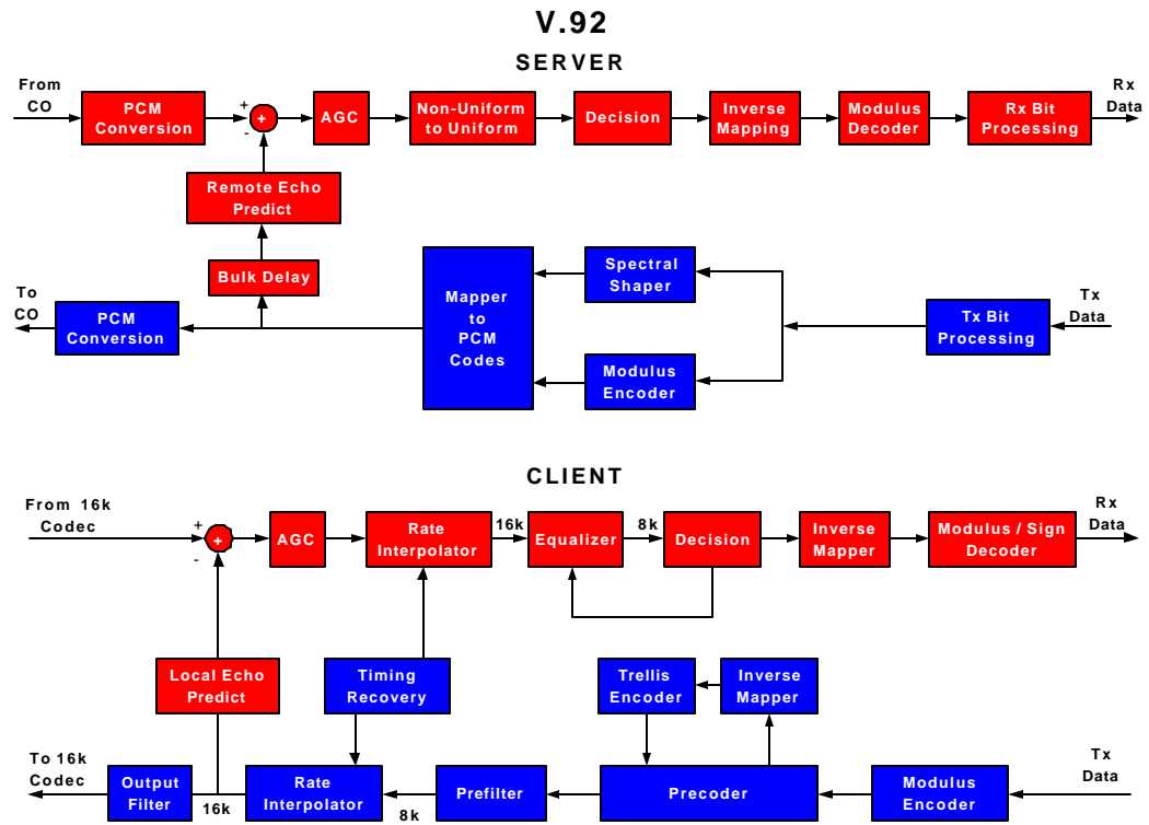
Figure 1 V.92 modem Server and Client
