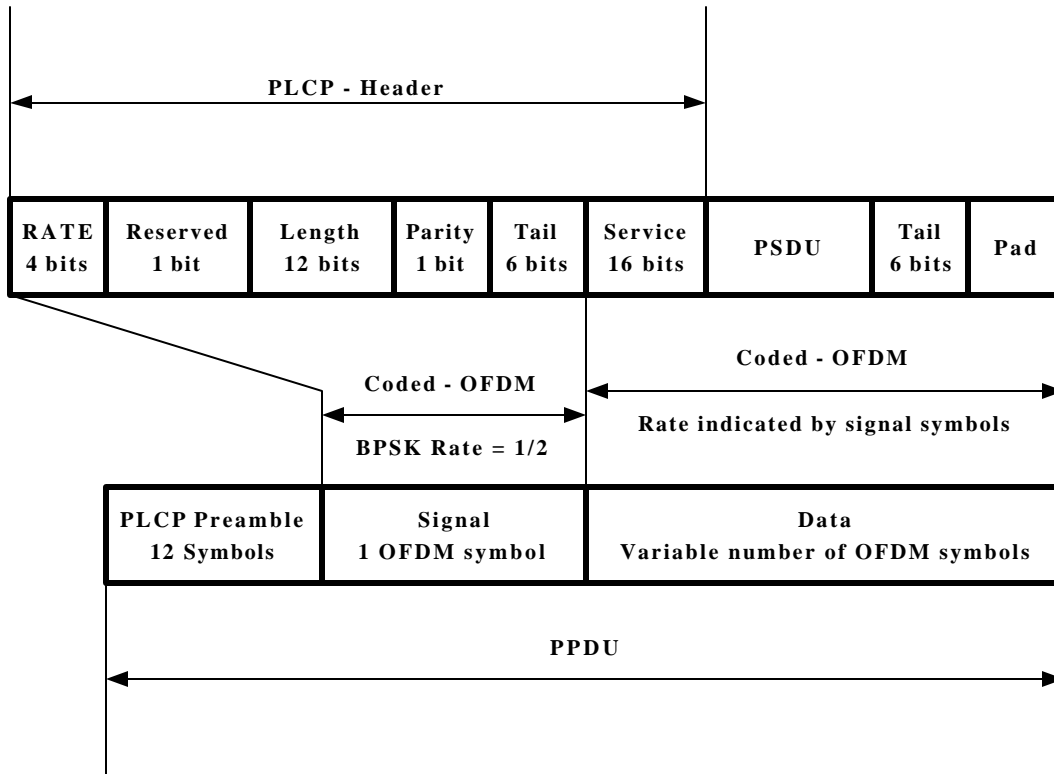
Figure 1. OFDM PLCP Preamble , Header and PSDU of 802.11a
