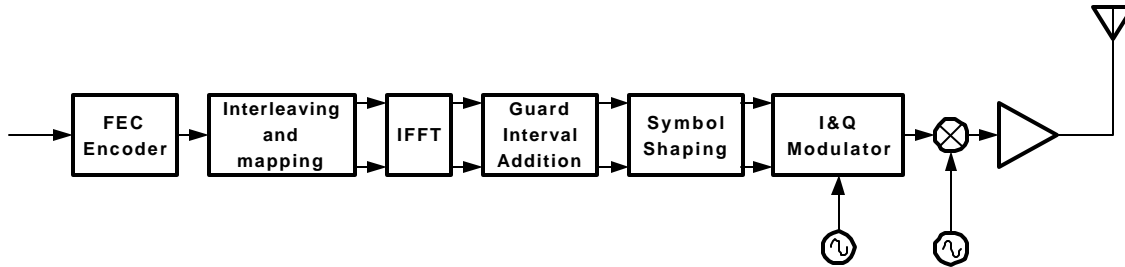
Figure 2. 802.11a Transmitter Block Diagram
